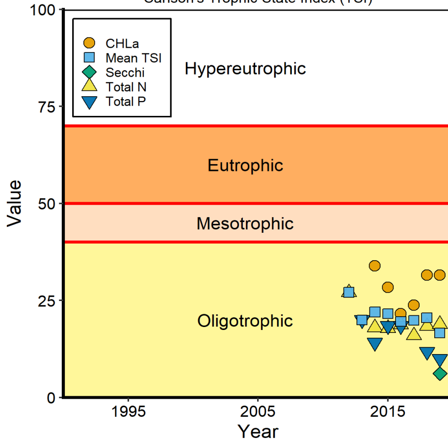
Carlson's Trophic State Index (TSI)
